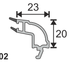
PRO702 24-26 mm Çiftcam Çıta 24-26 mm D.Glass Gazing Bead
