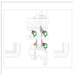
Glazing bead saw GLS 192 Our patented clamping device simulates the position of the installed glass pane when cutting the glazing beads
