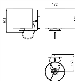
VICTORIAN COLLECTION: DINASTY - Applique
