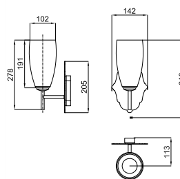
VICTORIAN COLLECTION: CENTURY - Aplique
