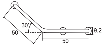
Assa parede 50x50 cm. 30°
